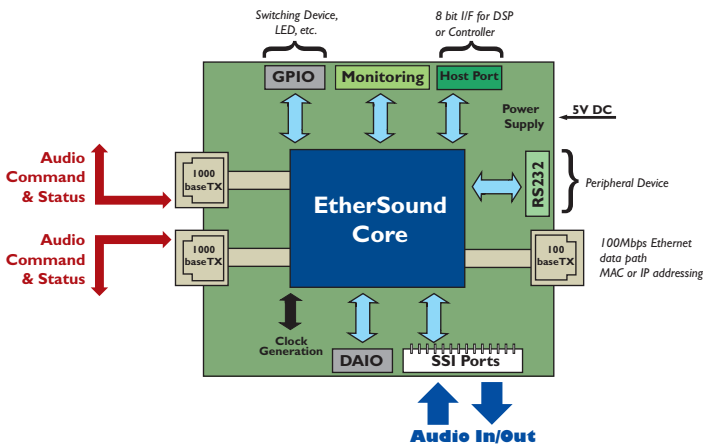
An example of an ES-Giga EtherSound implementation.
